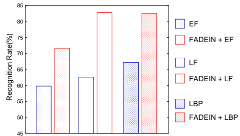
Fig. 8. Identification performance with and without FADEIN on FERET for artificial camera focus blur. Query set are blurred with Gaussian PSF.
