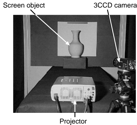
Figure 3: Prototype system.
