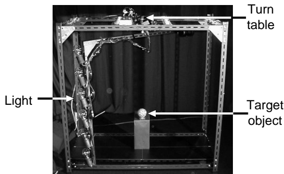
Figure 10: BRDF acquisition system.
